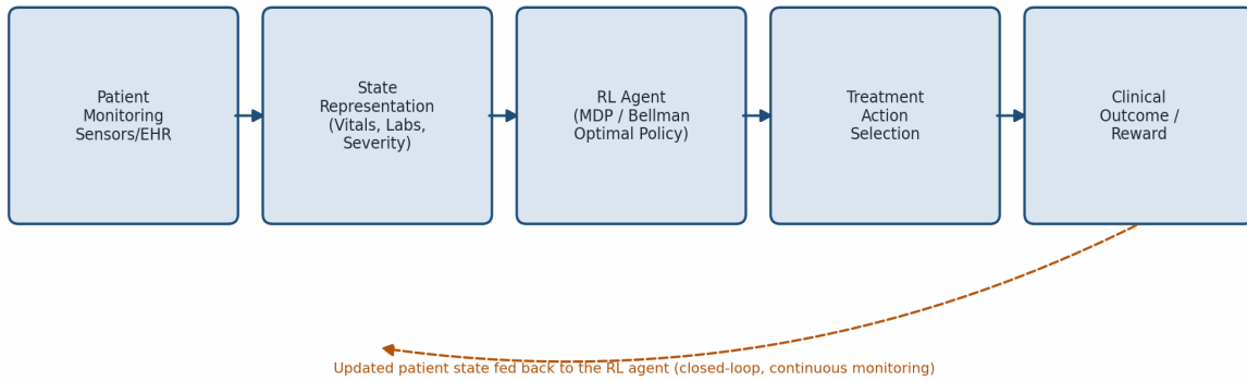
Figure 2: Closed-loop architecture connecting patient monitoring data, the RL agent, and clinical feedback.
